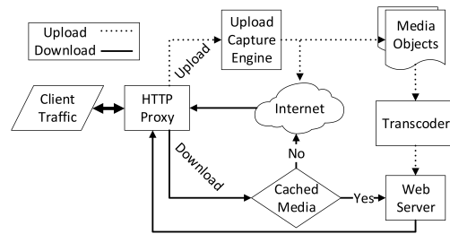
Figure 9: System architecture.
