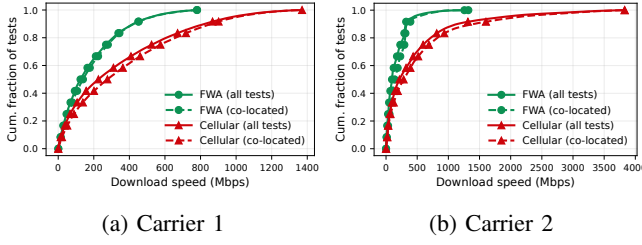
Fig. 7: Distribution of FWA and cellular performance for all tests vs co-located tests.
