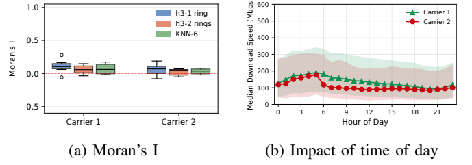
Fig. 6: Spatial and temporal influences on FWA speeds.
