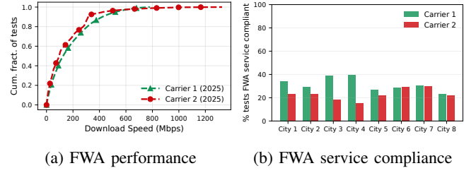
Fig. 4: 2025 FWA download speeds and measurements meeting FWA service threshold ( \geq 100/20 Mbps, \leq 100 ms).
