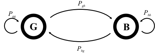
Fig. 2. Gilbert error model state diagram.
