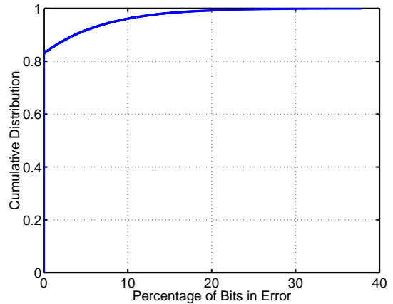
Fig. 10. Cumulative distribution function of packet bit errors when using the Interference Limited (IL) error model parameters.
