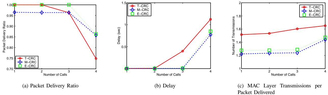
Fig. 9. Interference Limited (IL) error model results.
