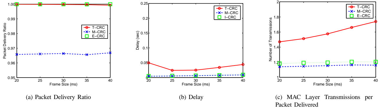
Fig. 8. Voice frame size results.
