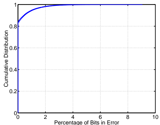
Fig. 6. Cumulative distribution function of packet bit errors.
