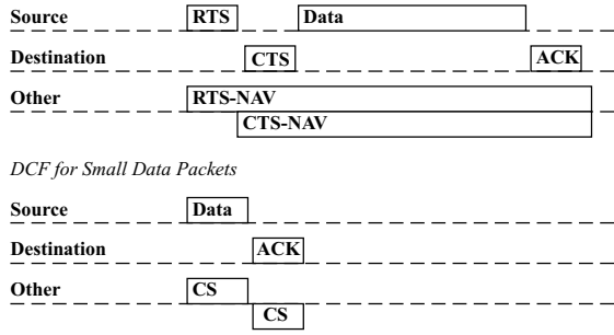
Fig. 1. IEEE 802.11 distributed coordination function.
