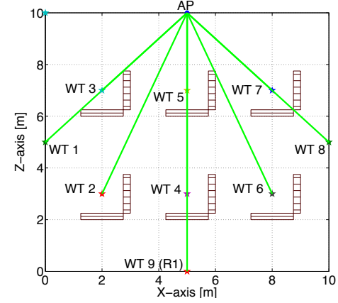
(b) Office
