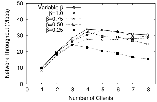
Fig. 10. Impact of \beta parameter.
